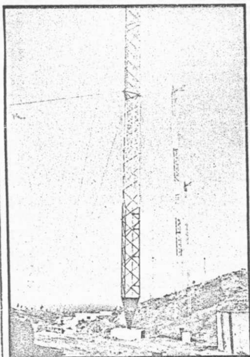
AWR-Asia as seen from the northernmost tower in antenna system two, still under construction.
